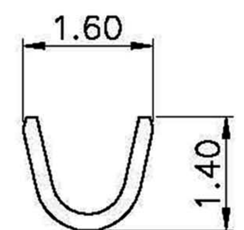
Section B-B
