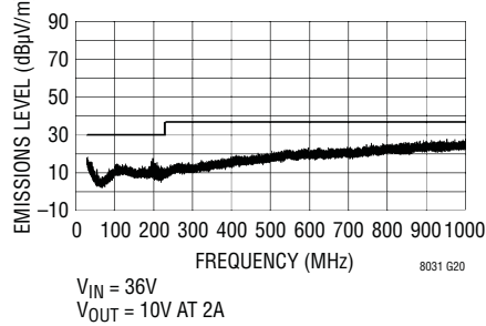
Radiated Emissions
