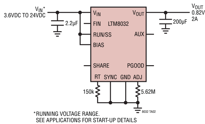
0.82V Step-Down Converter
