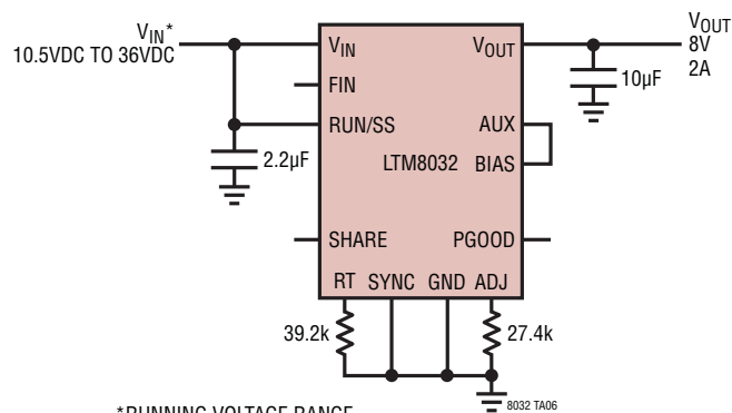
8V Step-Down Converter
