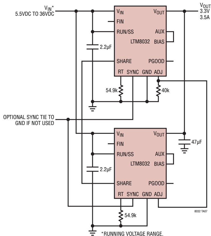
Two LTM8032s Operating in Parallel
