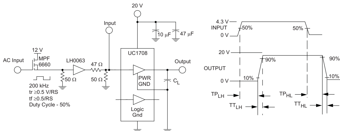
Figure 1. AC Test Circuit and Switching Time Waveforms
