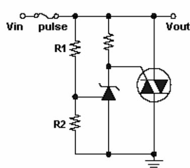
Figure 9. Crow Bar
