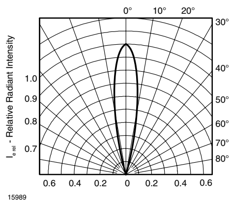
Figure 8. Relative Radiant Intensity vs. Angular Displacement
