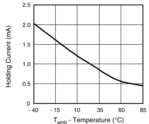
Fig. 10 - Normalized Holding Current vs. Temperature
